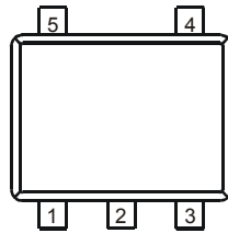
Pin Description (Top View)
